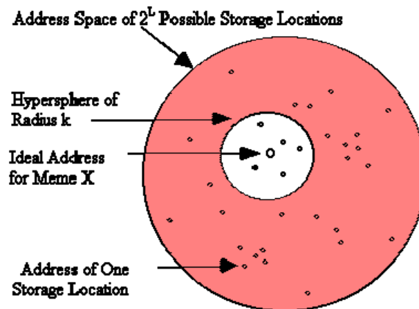
Figure 2: Meme X is stored in all locations within hypersphere of radius k surrounding its ideal address
